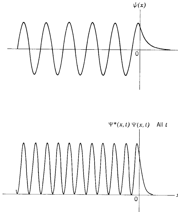
Figure 6-7 Top: The eigenfunction \psi(x) for a particle incident upon a potential step at x=0 , with total energy less than the height of the step. Note the penetration of the eigenfunction into the classically excluded region x > 0 . Bottom: The probability density \Psi^*\Psi = \psi^*\psi = \psi^2 corresponding to this eigenfunction. The spacing between the peaks of \psi^2 is twice as close as the spacing between the peaks of \psi .
